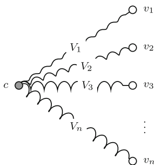
Fig. 4. If no two springs are equivalent, the v_i are controllable. Springs from the v_i to other particles or from one v_i to another may exist but are not shown. They do not change the conclusion
