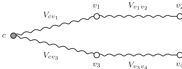
Fig. 7. The network used in Example 7.1. If V_{cv_3} is equivalent to V_{cv_1} our theory does not allow to conclude, but the network might still be controllable
