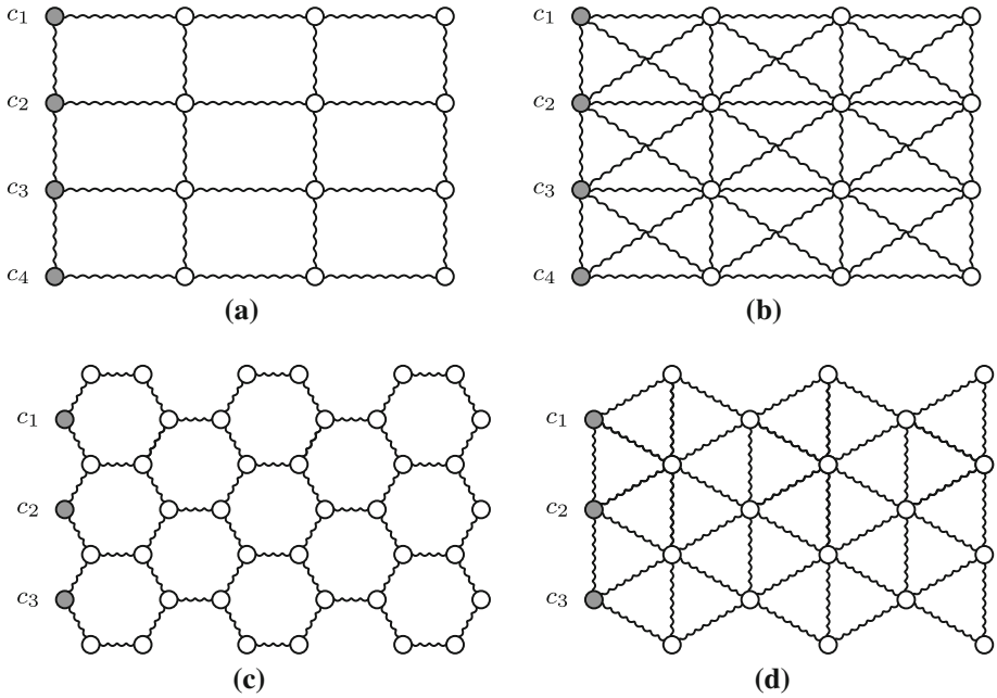
Fig. 6. Four networks that are controllable by their topology alone, regardless of the potentials (as long as they are polynomials of degree at least 3)
