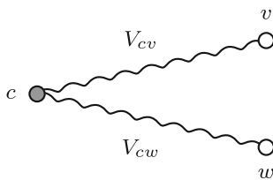
Fig. 8. The network discussed in Example 7.2
