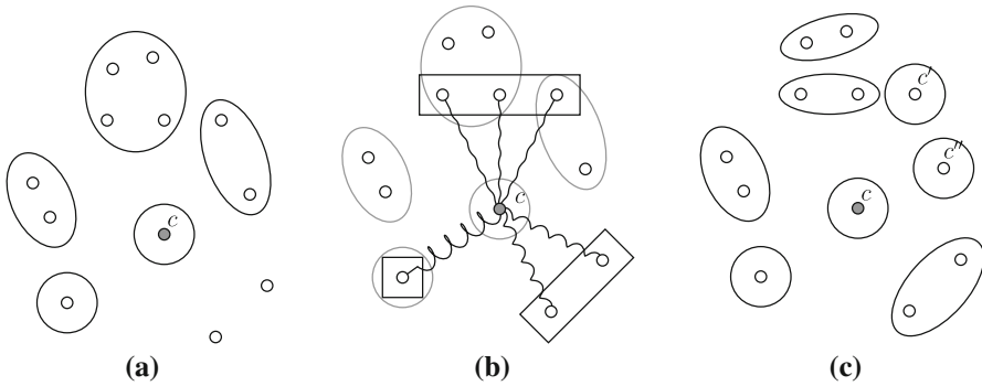
Fig. 1. a A controller c and a few sets in \mathcal{J} , shown as ovals. b The equivalence classes \mathcal{T}_i^c are shown as rectangles. (Only the edges incident to c are shown.) c New sets “appear” in \mathcal{J} . In particular, c' and c'' are controllable
