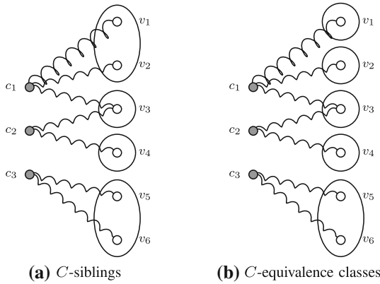
Fig. 2. Illustration of Definition 5.4. We assume that all the springs are identical, except for the edge \{c_1, v_1\} . The particles v_1, \dots, v_6 form 4 sets of C -siblings, with C = \{c_1, c_2, c_3\} . The one containing v_1 and v_2 is further split into two C -equivalence classes, since v_1 and v_2 are by assumption inequivalent with respect to c_1
