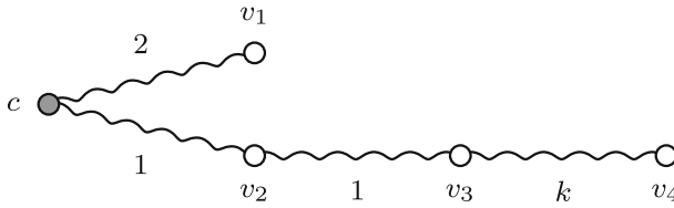
Fig. 9. A harmonic network that may or may not be controllable depending on the value of the coupling constant k
