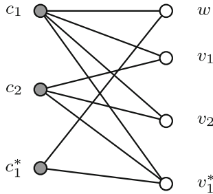
Fig. 3. Illustration of the proof of Proposition 5.5 for identical springs. We consider the C -equivalence class U = \{v_1, v_2\} , where C contains c_1, c_2, c_1^* and possibly other particles (not shown) that are not linked to v_1, v_2 . With the notation of the proof, we have \mathcal{S}_1 = \{w, v_1, v_2, v_1^*\} and \mathcal{S}_2 = \{v_1, v_2, v_1^*\} so that \widehat{U} = \mathcal{S}_1 \cap \mathcal{S}_2 = \{v_1, v_2, v_1^*\} . Since v_1^* belongs to \mathcal{S}_1^* = \{w, v_1^*\} , we find \widehat{U} \setminus \mathcal{S}_1^* = U
