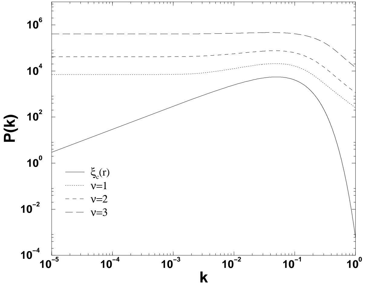
Fig. 1.— The PS P_\nu(k) derived from the biased correlation function \xi_\nu(r) for values of the threshold \nu = 1, 2, 3 is shown. The underlying correlation function which gives \xi_c(r) is that derived from the P(k) = Ake^{-k/k_c} and the approximation given in Eq. (10) for \xi_\nu is used. The clear distortion of the PS at small k is seen, the “turn-over” in the underlying PS essentially disappears already for \nu = 1 . The constants k_c and A are fixed by \xi_c(0) = 1 and the requirement that \xi_c(r) = 0 at r = 38 Mpc. The latter is taken as in a typical CDM model (see e.g. Padmanabhan 1993). We could alternatively fix the wavenumber at the maximum of the PS.
