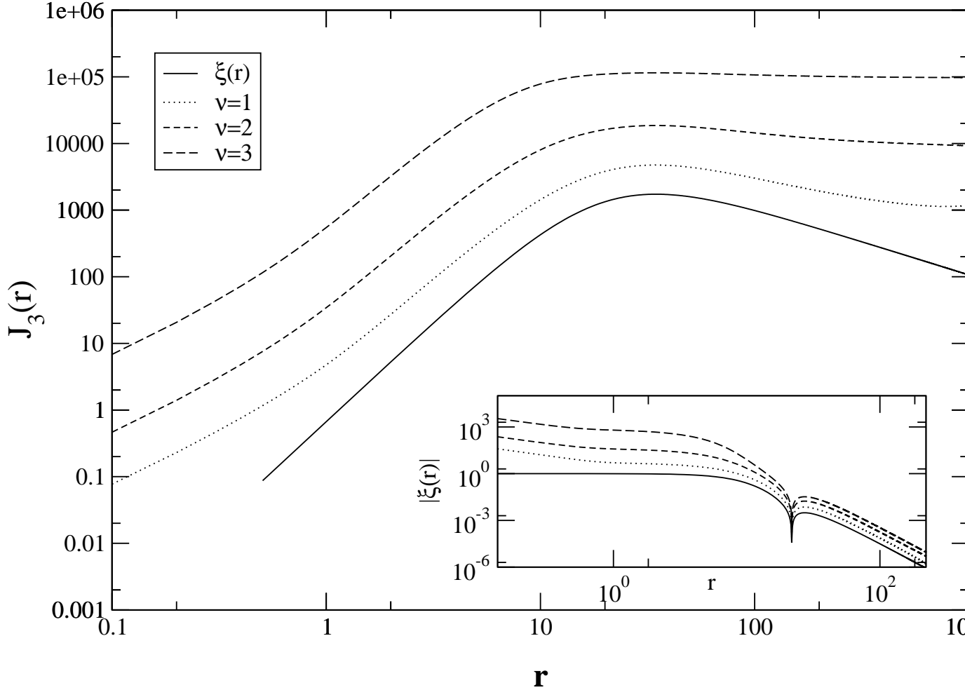
Fig. 2.— The integral J_3(r) for the same underlying correlation function as in Figure 1 and for the same range of values of \nu , calculated with the exact expression Eq. (4) for \xi_\nu(r) . Also shown is the analogous integral of \xi_c . While the latter converges slowly to its asymptotic value of P(0) = 0 , the other integrals converge to constant non-zero P_\nu(0) . They are dominated by the range r \sim 10 Mpc where, as can be seen from the inset which shows both \xi_c and each of the \xi_\nu(r) , the correlation functions \xi_\nu(r) are amplified non-linearly. The contribution from the extremely amplified region at small r is small (because of the r^2 factor in the integral), which also makes the approximation in calculating the PS with Eq. (10) very accurate, as can be checked by comparing the asymptotic values with those of P_\nu(0) in Figure 1.
